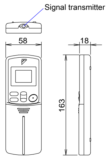
Remote control | Infrared type (ARC433A87)
